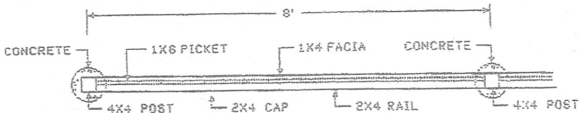
(PLAN VIEW)
