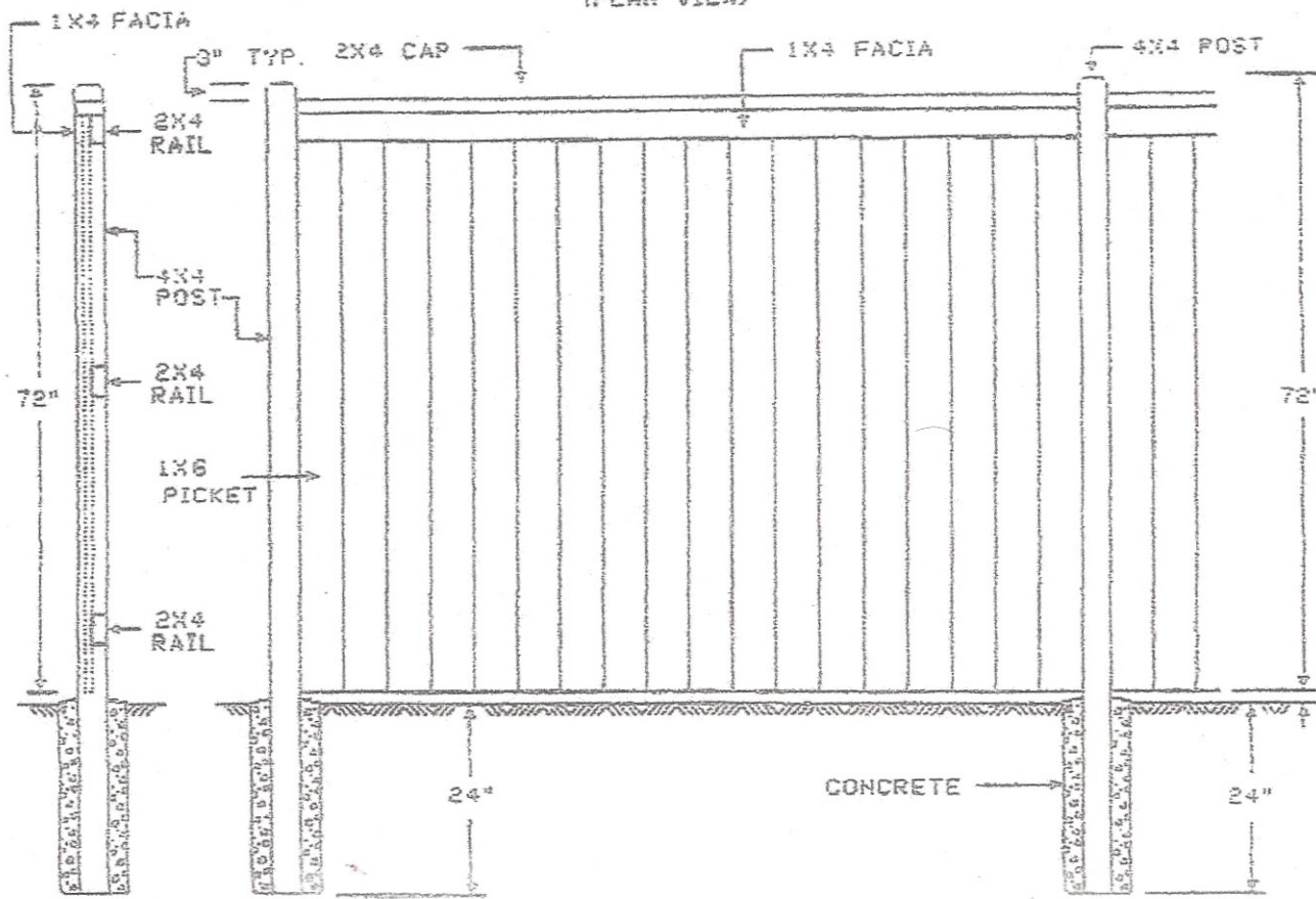
(ELEVATION VIEW)
